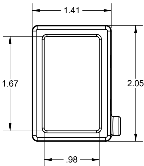
GDS SERIES (SQUARE PLASTIC CASE)
